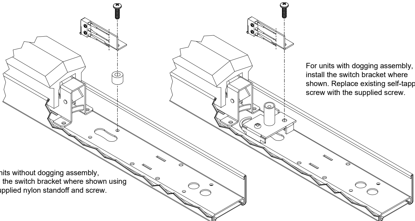
531 SWITCH KIT
