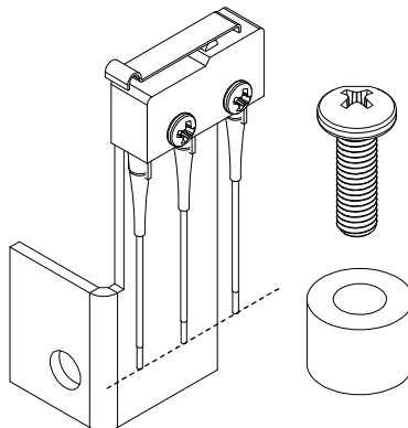
531 SWITCH KIT
