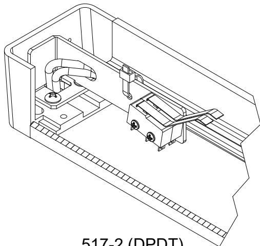
517-2 (DPDT) CONTAINS TWO SWITCHES
