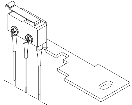
511 SWITCH KIT
